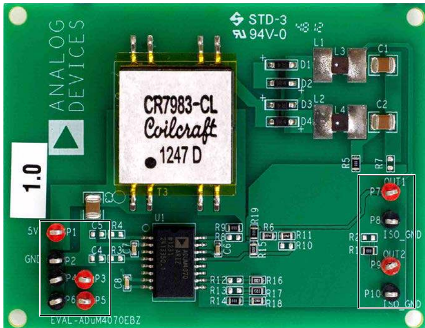
Figure 2. Single-Supply and Double-Supply Board Terminals
