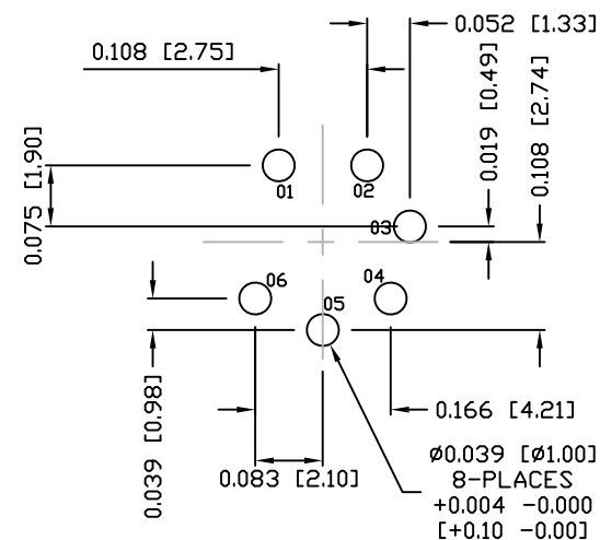
PCB LAYOUT
