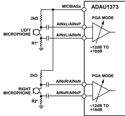
*R1 AND R2 CAN BE 2k \Omega FOR DIFFERENTIAL OR \infty\Omega FOR PSEUDO-DIFFERENTIAL INPUT.
