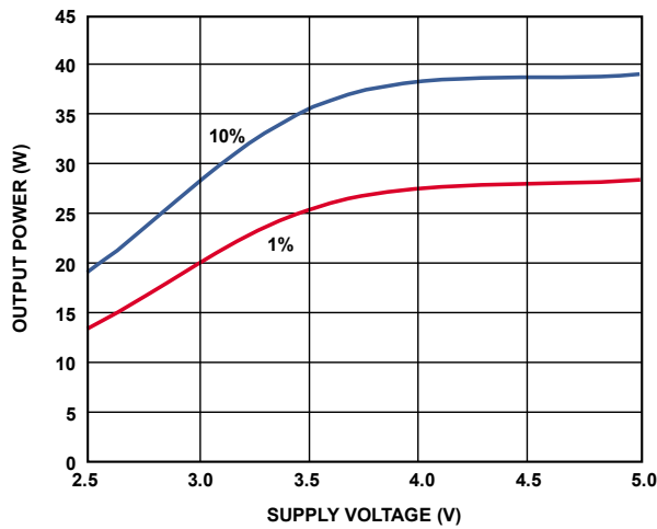
Figure 59. Output Power vs. SPKVDD, 32 \Omega , Digital In \rightarrow Earpiece Out
