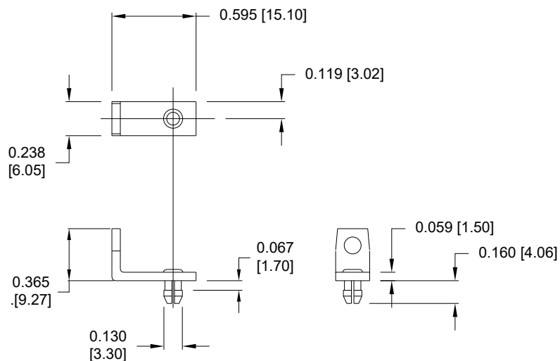
MOUNTING BRACKET WITH BOARD LOCK
