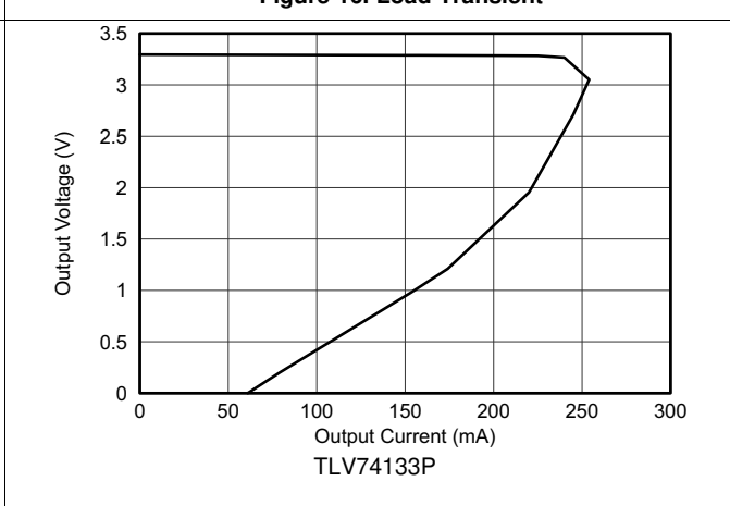
Figure 18. 3.3-V Output Voltage vs Output Current (Foldback Current Limit)
