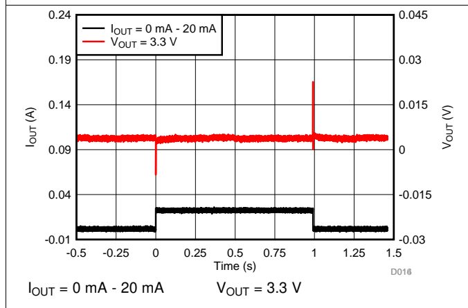
Figure 15. Load Transient
