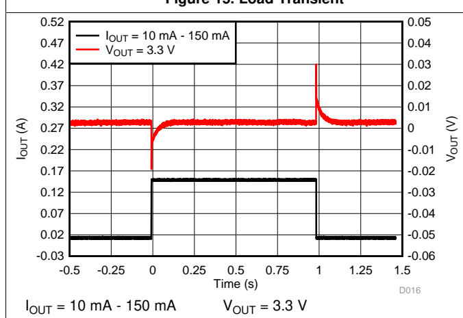
Figure 17. Load Transient
