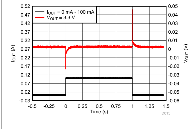
Figure 16. Load Transient
