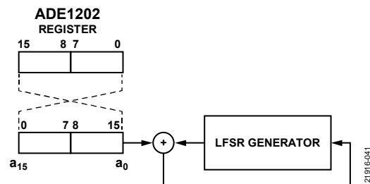
Figure 45. CRC Calculation
