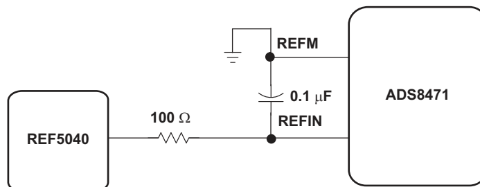
Figure 38. ADS8471 Using External Reference
