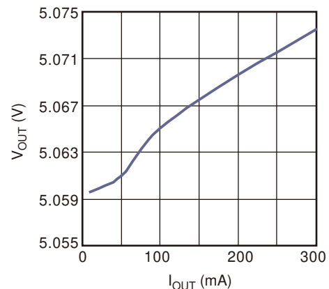
V_{OUT} vs. I_{OUT} V_{IN}=6\text{V}
