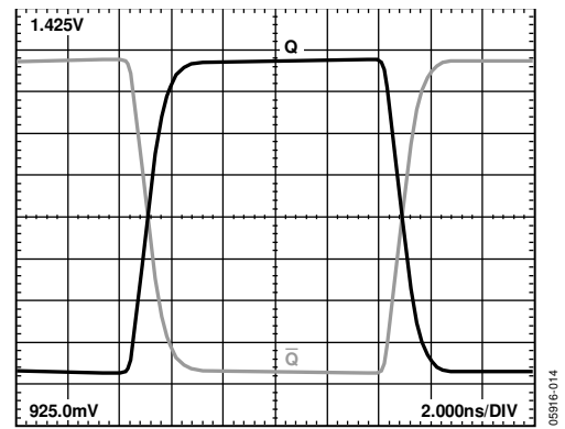
Figure 15. 50 MHz Output Voltage Waveform at V_{CC0} = 2.5 V
