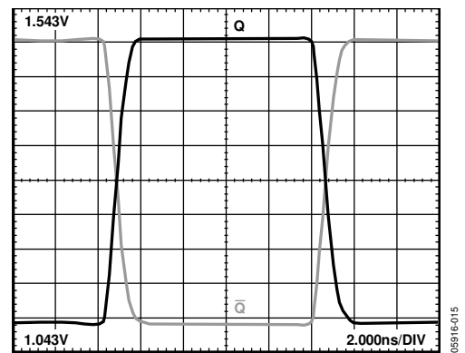
Figure 16. 50 MHz Output Voltage Waveform at V_{CC0} = 5 V
