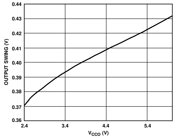
Figure 14. LVDS Output Swing vs. V_{CC0} (V)
