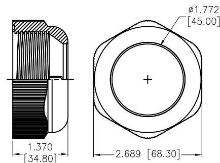
Ⓔ Sealing Nut
