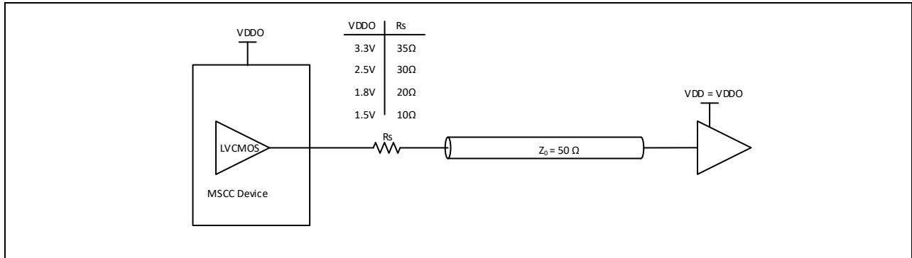
Figure 11. Termination for LVC MOS outputs
