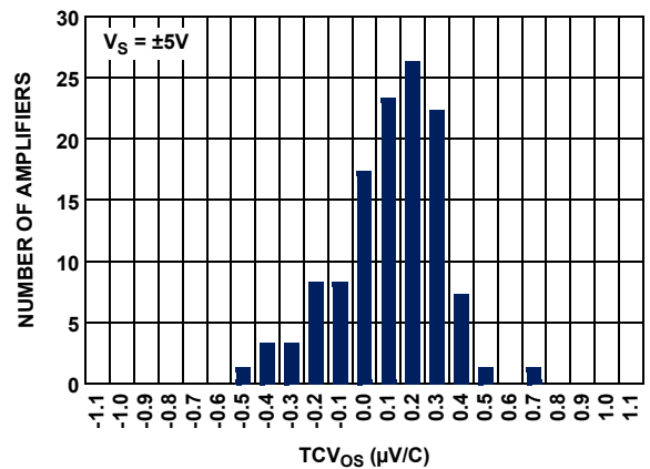
FIGURE 18. ISL28108 SOIC TCV_{0S} vs NUMBER OF AMPLIFIERS, V_S = \pm 5V
