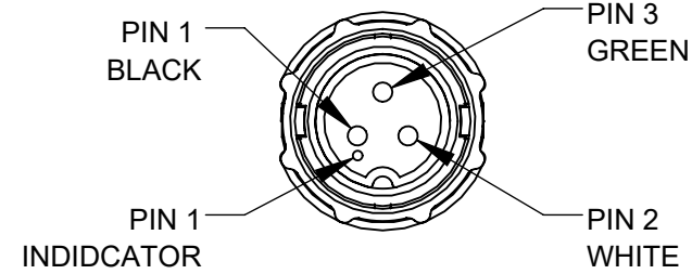
CAEN3C3M1607990 3-PIN MALE
