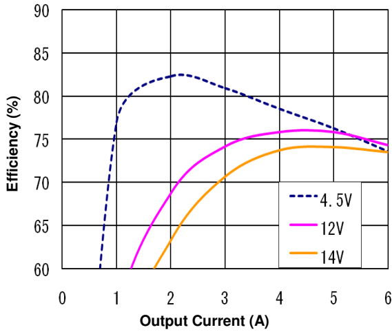
Figure 1(a). Efficiency vs. Load Current (25°C, 0.59V output)
