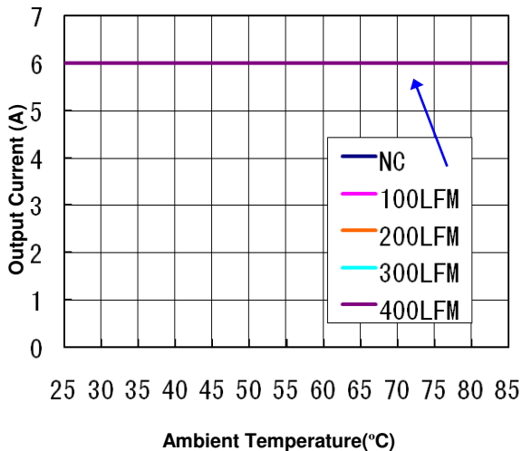
Figure 8(e). Current Derating Curve for 3.3V Output Vin = 12V, open frame
