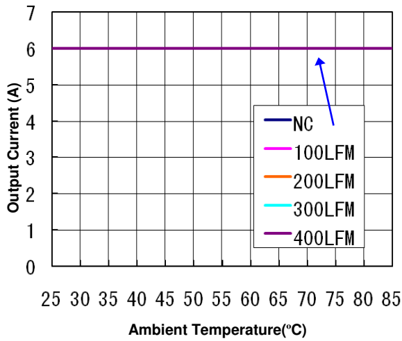
Figure 8(a). Current Derating Curve for 0.59V Output Vin = 12V, open frame Output
