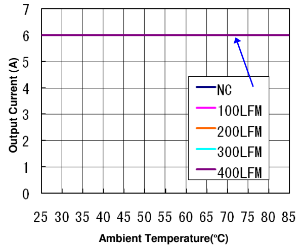
Figure 8(d). Current Derating Curve for 2.5V Output Vin = 12V, open frame
