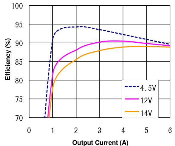
Figure 1(d). Efficiency vs. Load Current (25°C, 2.5V output)
