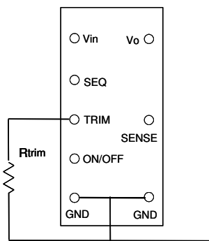
Figure 12. Circuit to Trim Output Voltage.
