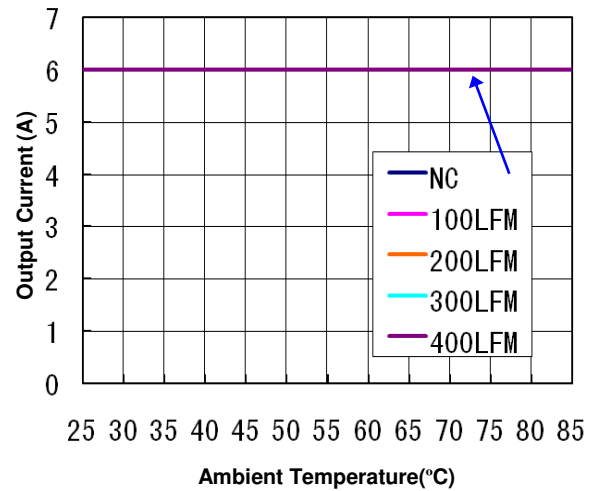
Figure 8(b). Current Derating Curve for 1.2V Output Vin = 12V, open frame
