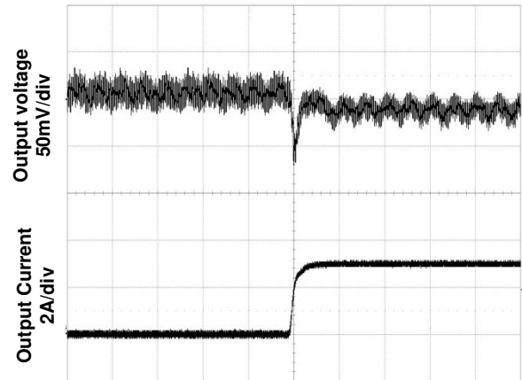
Figure 3. Transient Load Response. Input voltage 12V, Output voltage 5V, Output current 0A -> 3A, Slew rate 1A/μs
