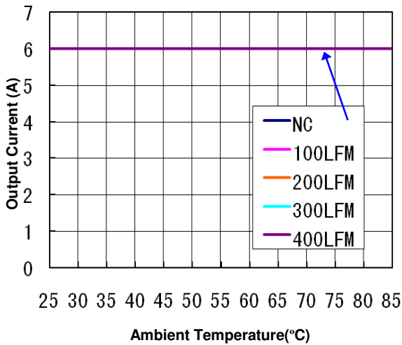
Figure 8(c). Current Derating Curve for 1.8V Output Vin = 12V, open frame
