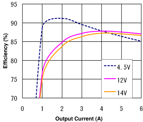
Figure 1(C). Efficiency vs. Load Current (25°C, 1.8V output)
