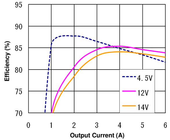
Figure 1(b). Efficiency vs. Load Current (25°C, 1.2V output)
