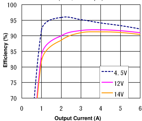
Figure 1(e). Efficiency vs. Load Current (25°C, 3.3V output)
