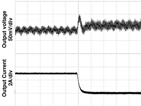
Figure 2. Transient Load Response Input voltage 12V, Output voltage 5V, Output current 3A->0A, Slew rate 1A/μs
