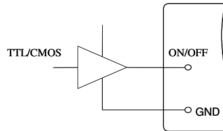
Figure 10. Direct Logic Drive
