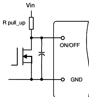
Figure 9. Circuit for Logic Control
