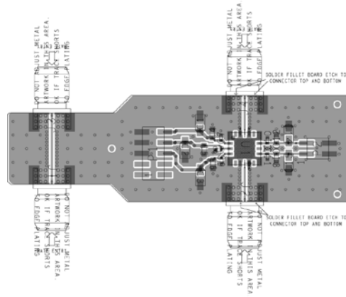
Figure 5. EV1HMC8342LS6 Silk Screen and Metal 1, Top Side
