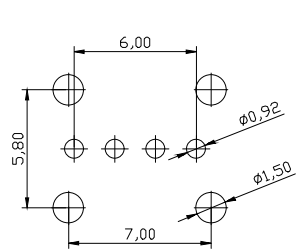
RECOMMENDED PCB LAYOUT(TOP VIEW) GENERAL TOLERANCES:±0.05
