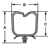
WWS Push Mount Type
