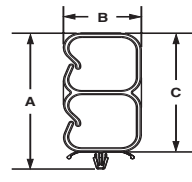
VVSDC Dual Capacity Type
