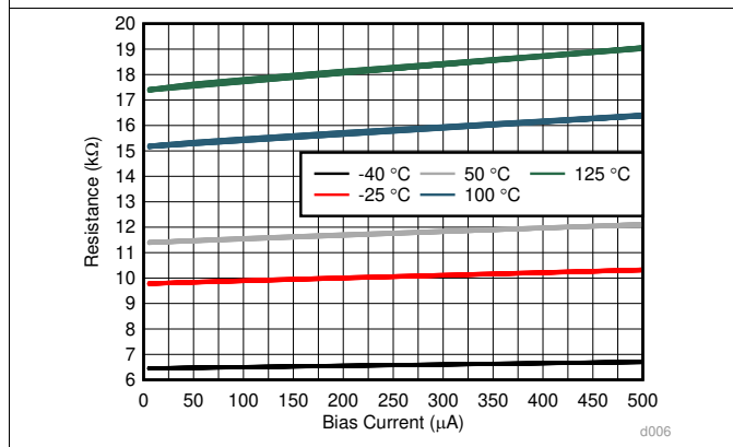
Figure 5. Supply Dependence Resistance vs. Bias Current
