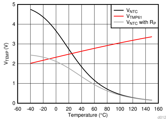
Figure 21. NTC With and Without a Linearization Resistor vs. TMP61 Temperature Voltages
