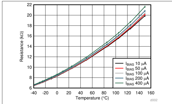
Figure 1. Resistance vs. Ambient Temperature Using Multiple Bias Currents
