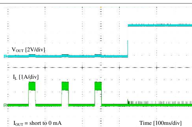
Figure 9-9. Short Recovery
