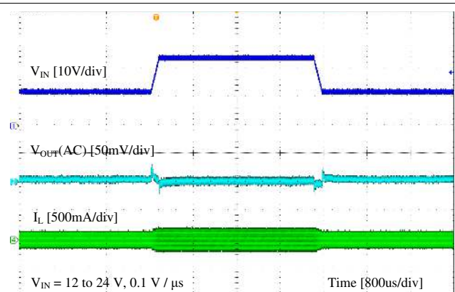
Figure 9-7. Line Transient
