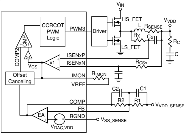
Figure 8. VDD Controller : Simplified Schematic for Droop and Remote Sense in CCM
