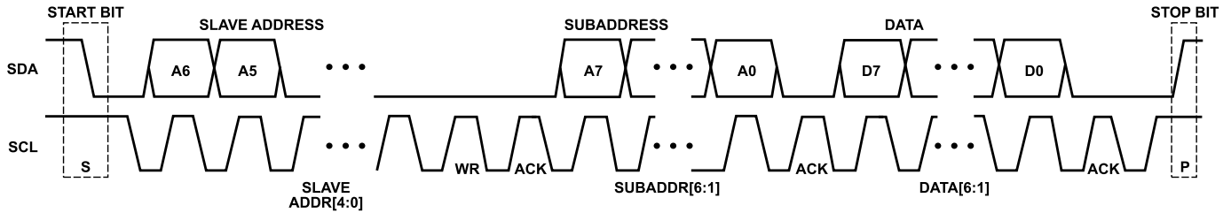
Figure 64. I 2 C Data Transfer Timing
