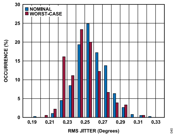
Figure 40. Integrated Phase Noise Distribution with LO Frequency = 1000 MHz at Nominal and Worst-Case Conditions
