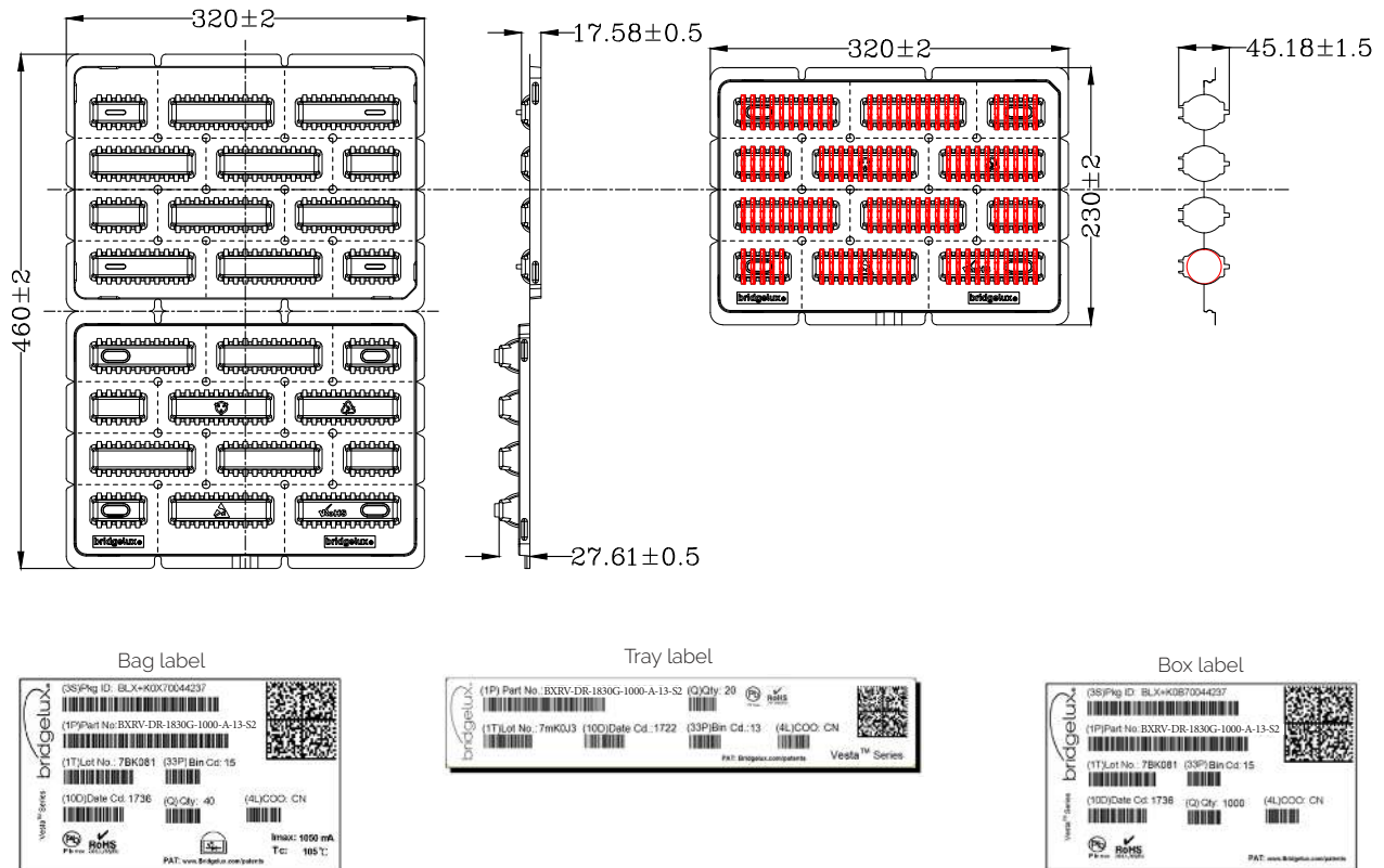
Figure 14: Packaging Specifications
