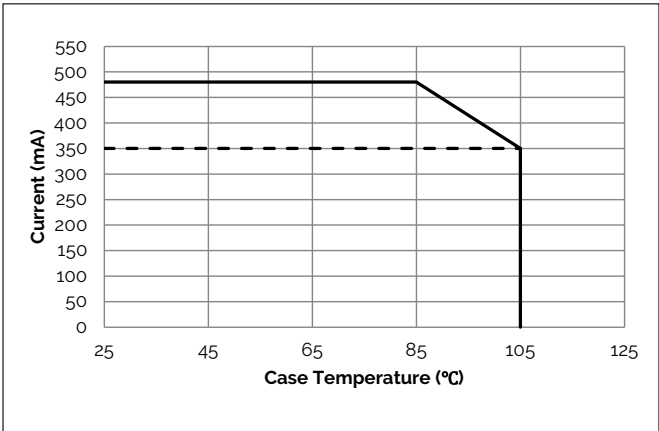
Figure 8: Derating Curve
