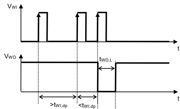
Figure 11 Watchdog Double-pulse Detection Time
