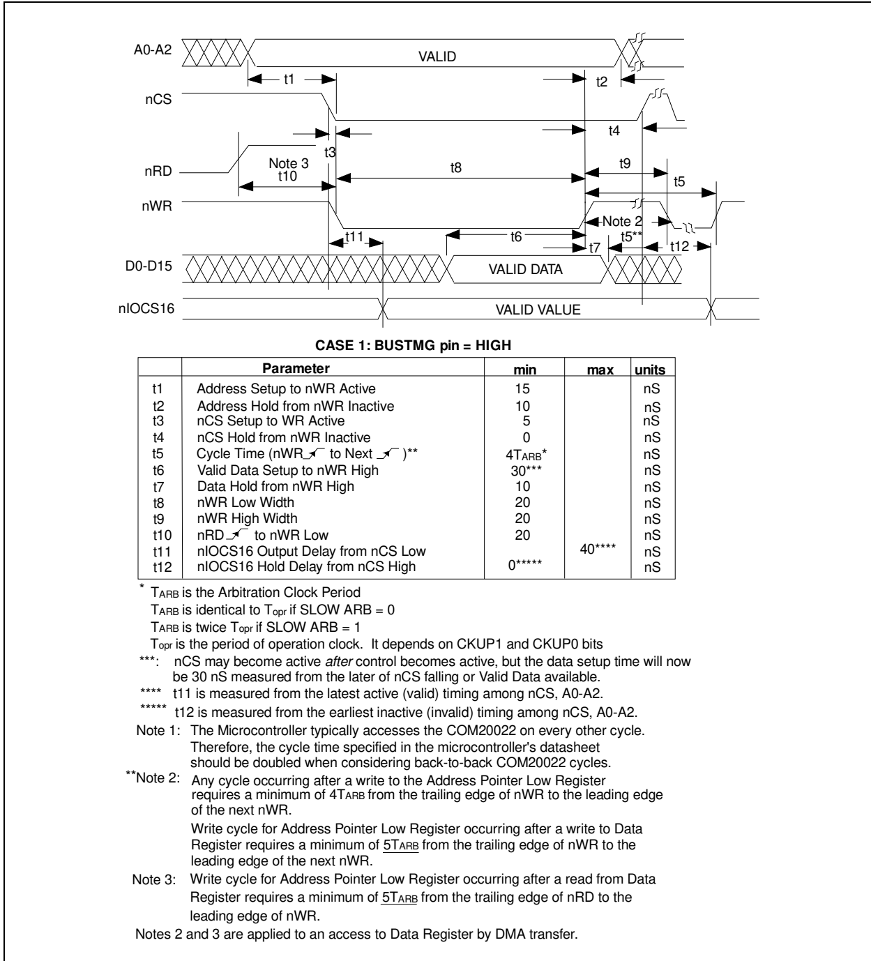
FIGURE 8-9: NON-MULTIPLEXED BUS, 80XX-LIKE CONTROL SIGNALS; WRITE CYCLE
