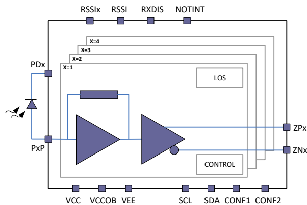
Figure 1: Device diagram
