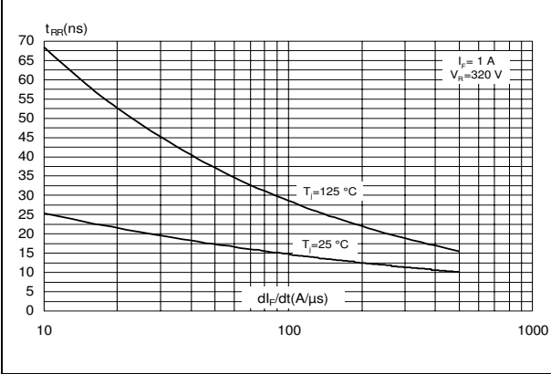
Figure 7: Reverse recovery time versus di_F / dt (typical values)
