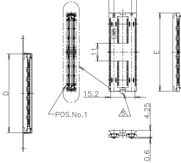
CONNECTOR DETAIL
