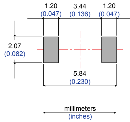
Figure 8. Footprint recommendations, dimensions in mm (inches)
