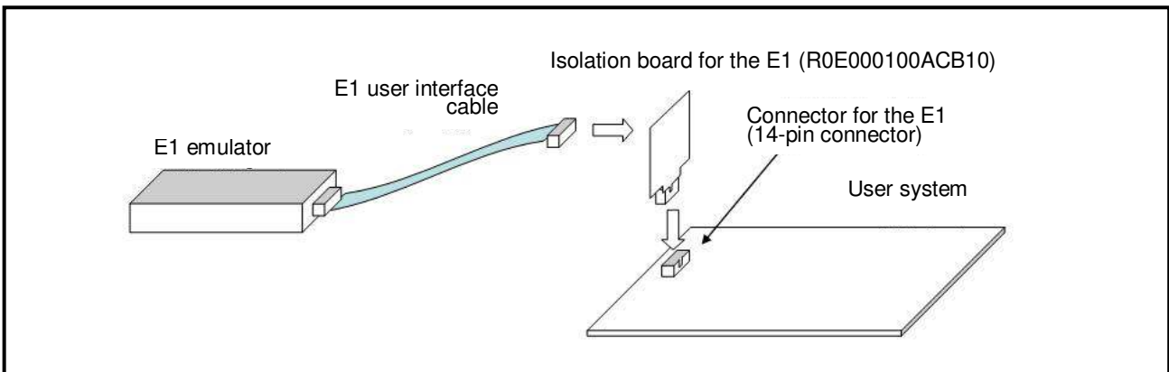
Figure 4.1 Mounting the R0E000010ACB10
