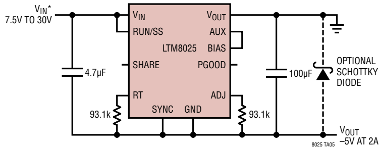
-5V Negative Output Converter
