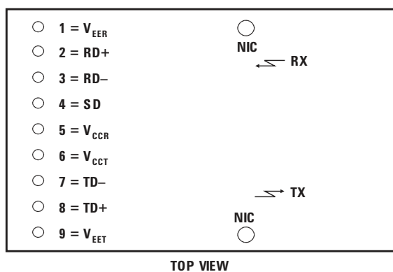
Figure 2. Pin-out.
