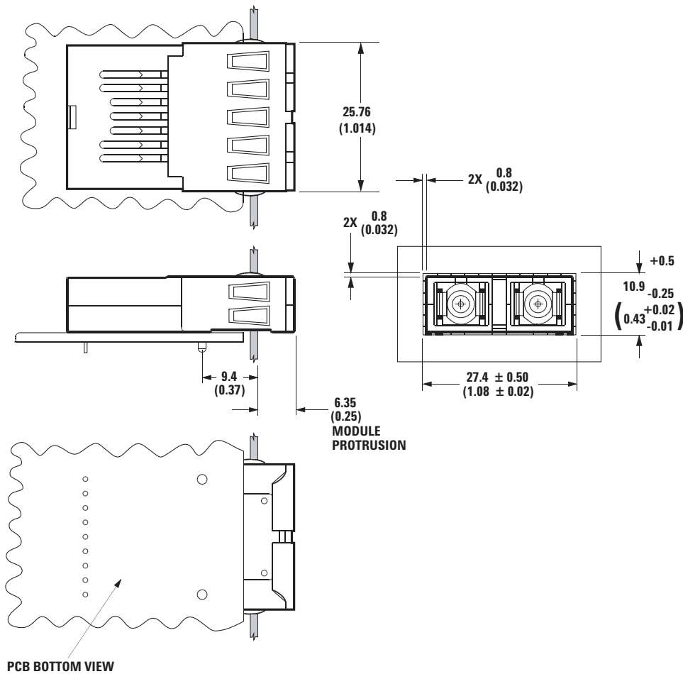
Figure 6. Suggested module positioning and panel cut-out for AFBR-53B3EZ.
