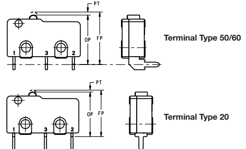
Operate Point References for PCB Terminals
