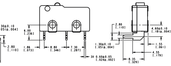
Terminal Type 60 - Left PCB
