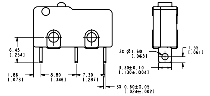
Terminal Type 20 - Straight PCB
