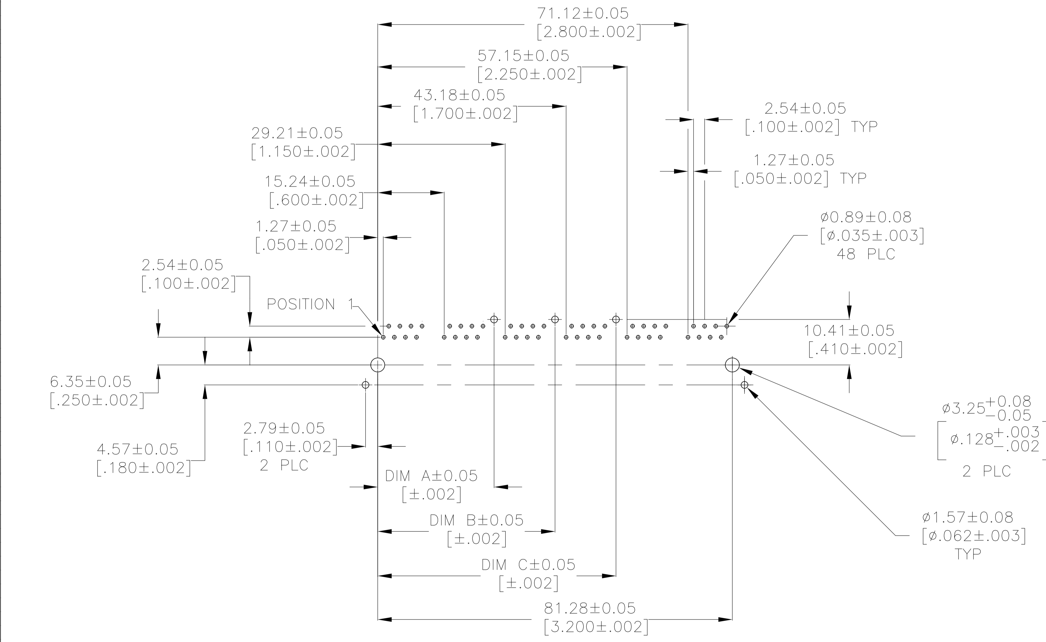
RECOMMENDED PC BOARD LAYOUT COMPONENT SIDE SCALE 2:1
