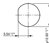
パネル取付穴寸法 (参考) (パネル厚: 1~4mm) PANEL MOUNTING HOLE PATTERNS (REF.) (PANEL THICKNESS : 1 to 4mm)
