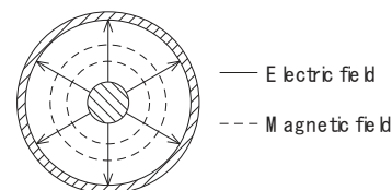
Direction of electromagnetic field in a coaxial line
