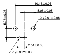
基板取付穴寸法 (参考・装着面) PC BOARD LAYOUT · MOUNTING SIDE (REF.)
