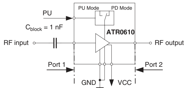
Figure 6-9. Reference Planes of Unmatched Device
