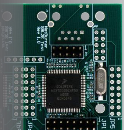
BOB Version with break out board
