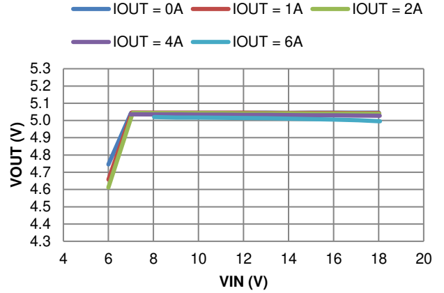
Figure 24. Line Regulation
