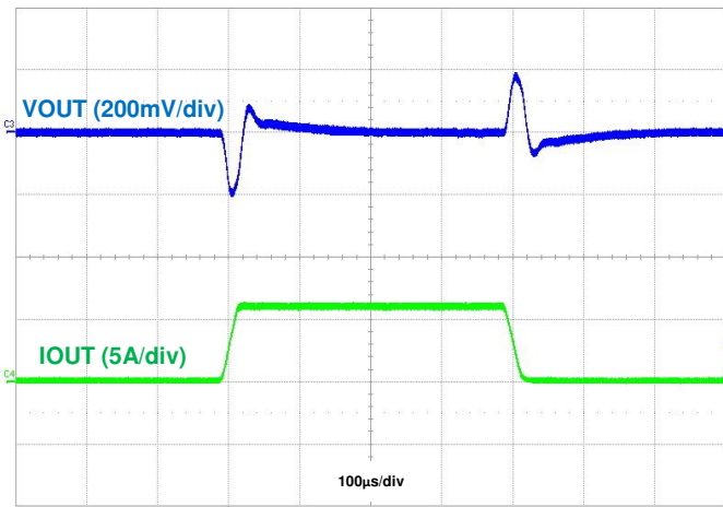
Figure 44. Load Transient, IOU = 50mA to 6A to 50mA
