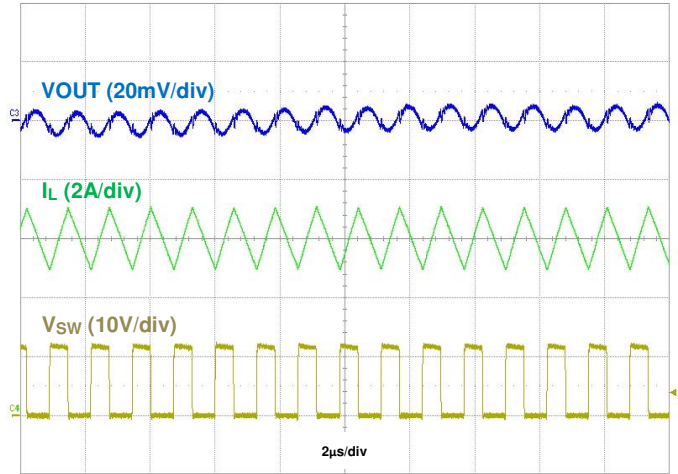
Figure 41. Output Voltage Ripple, IOU = 6A
