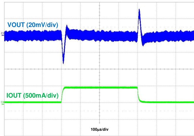
Figure 42. Load Transient, IOU = 50mA to 500mA to 50mA
