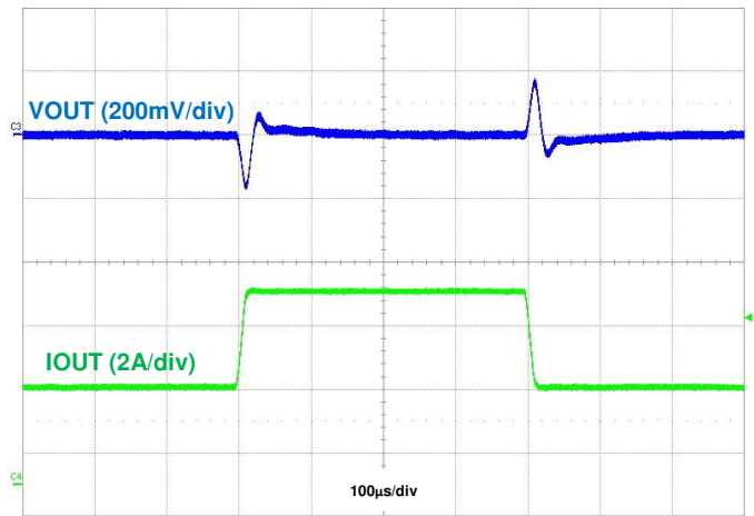
Figure 43. Load Transient, IOU = 3A to 6A to 3A
