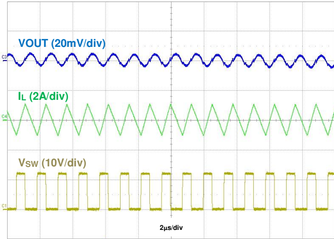
Figure 40. Output Voltage Ripple, IOU = 50mA
