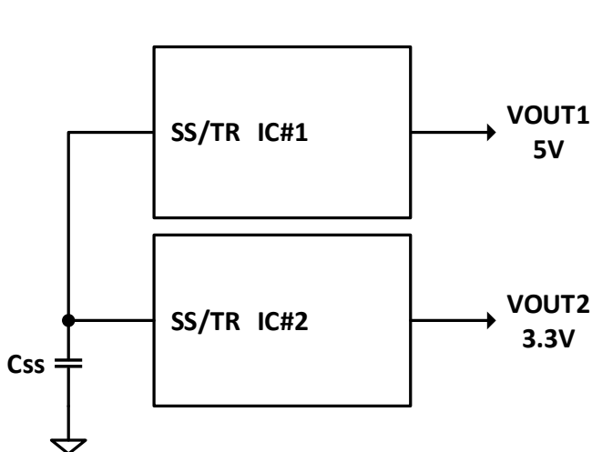
Figure 45. Ratiometric Tracking Configuration
