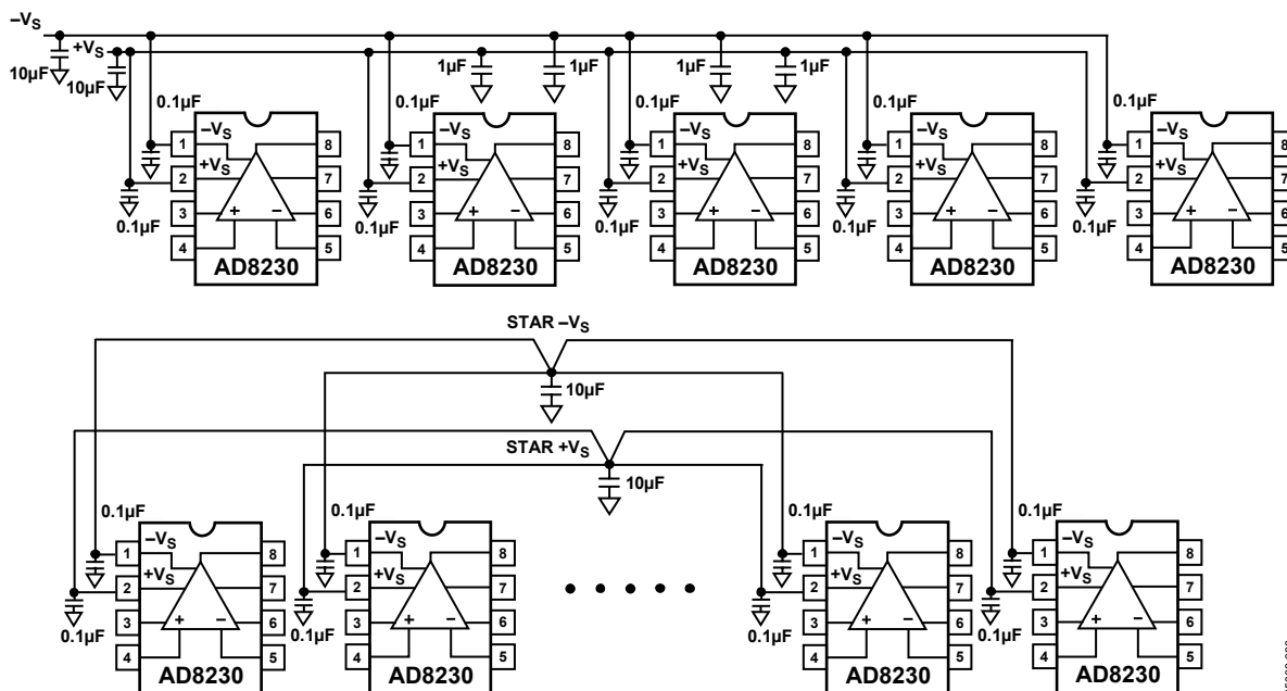
Figure 38. Use Star Nodes for +Vs and -Vs or Use Thick Traces and Decouple Frequently Along the Supply Lines
