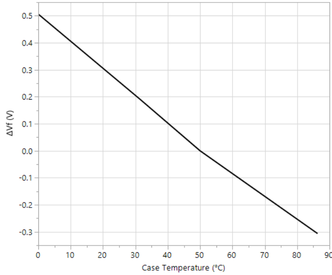
Figure 06: Forward voltage vs temperature (Measured at I_f = 2.5A and normalized at T_{case} = 50^\circ C )
