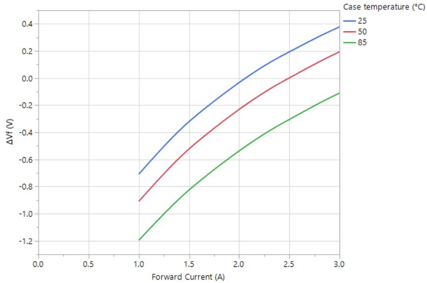
Figure 07: Change in forward voltage vs forward current (Normalized to at I_f = 2.5A and T_{case} = 50^\circ C )
