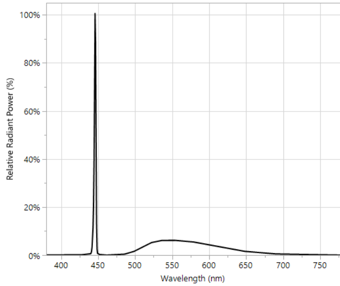
Figure 02: Typical spectral power distribution of 6500K component ( I_f = 2.5A , T_{case} = 50^{\circ}C )
