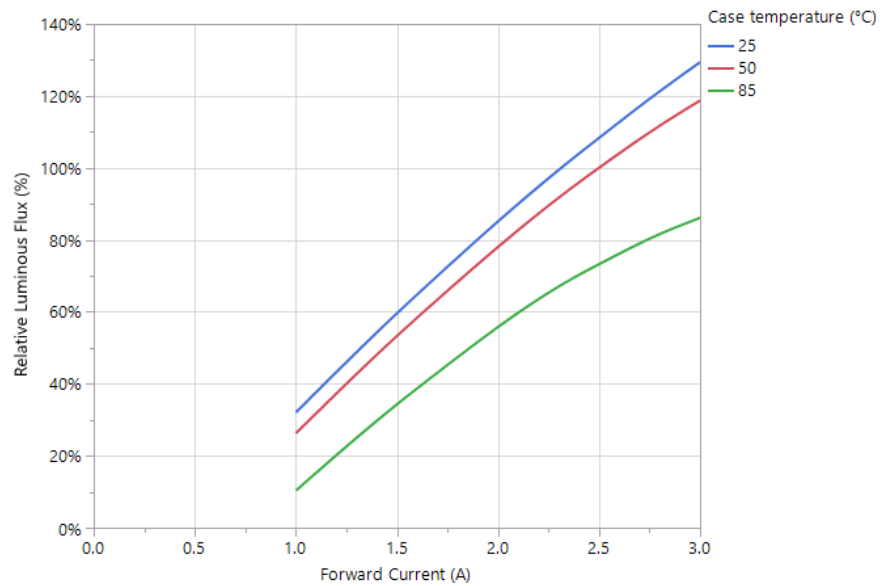
Figure 03: Relative flux vs forward current (Normalized to at I_f = 2.5A and T_{case} = 50^{\circ}C )
