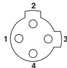
Pin assignment 1/2"-20UNF socket, 4-pos., view female side
