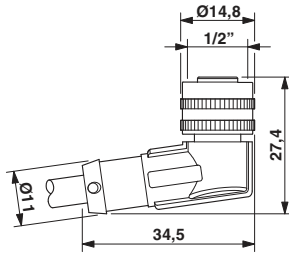
1/2"-20UNF socket, angled
