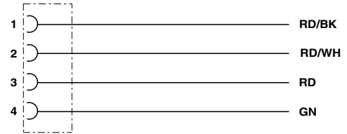
Contact assignment of 1/2" UNF sockets
