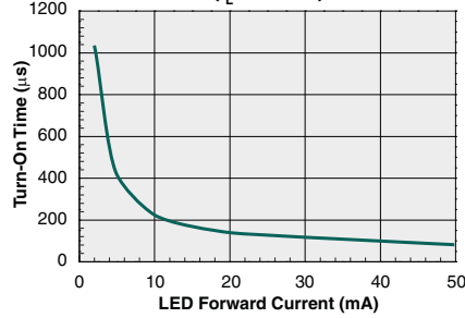
Form-A Typical Turn-On Time vs. LED Forward Current ( I_L=100\text{mA} )
