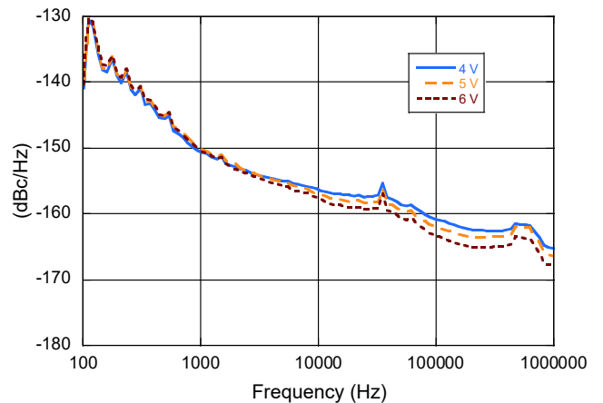
Phase Noise @ 12 GHz, P4dB
