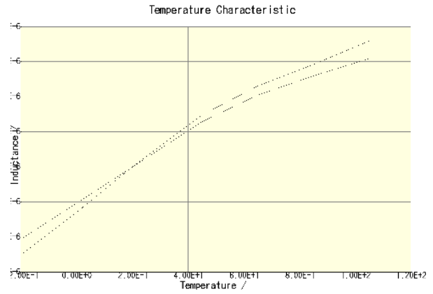
CLF7045T-3R3N-CA(DC = 0A)
