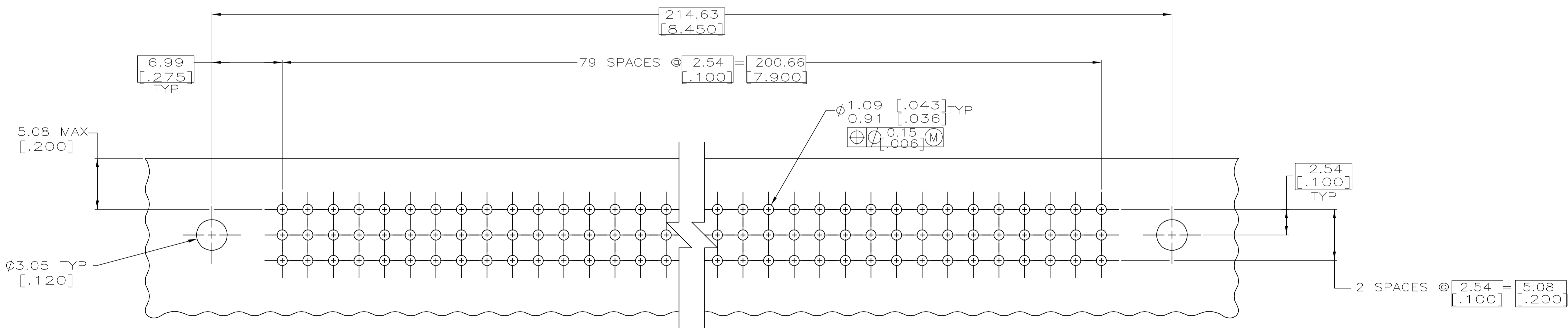
RECOMMENDED P. C. BOARD LAYOUT
