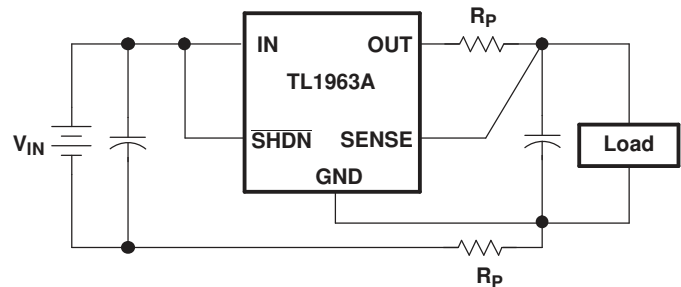
Figure 32. Kelvin Sense Connection
