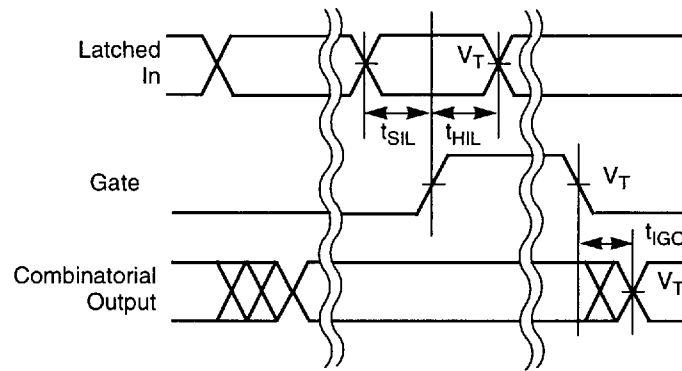
Latched Input
