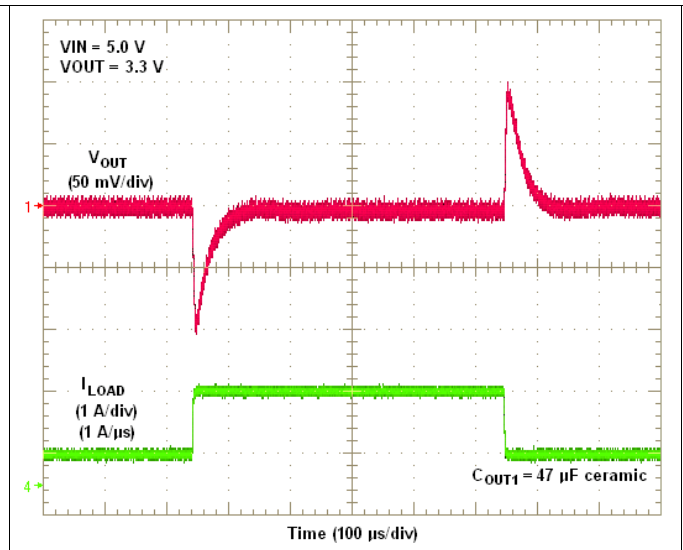
Figure 18. VIN = 5V, VOUT = 3.3V, 1A Load Step
