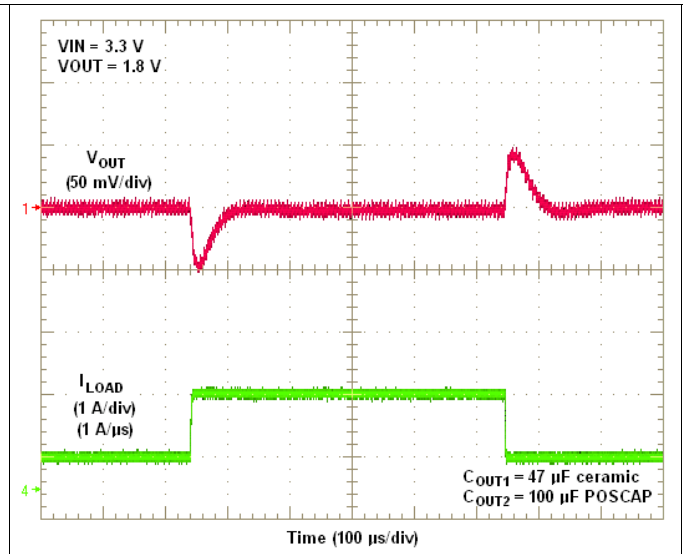
Figure 16. VIN = 3.3V, VOUT = 1.8V, 1A Load Step
