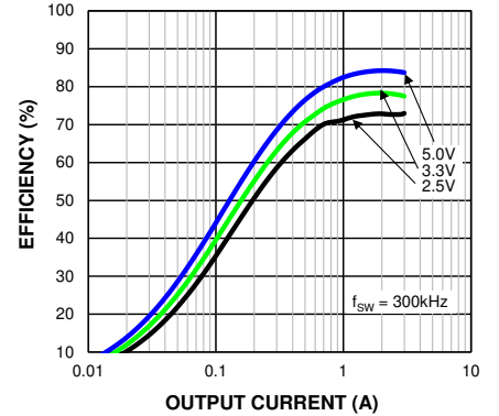
Efficiency (VIN = 48V) vs. Output Current MIC28511-2
