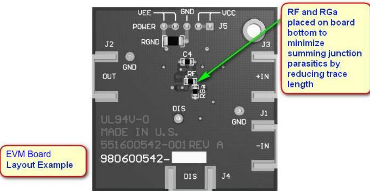
Figure 59. LM8261 Evaluation Board Layer 2
