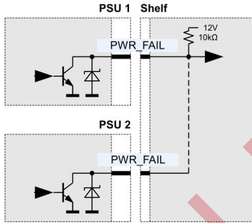
Figure 21. PWR_FAIL connection
